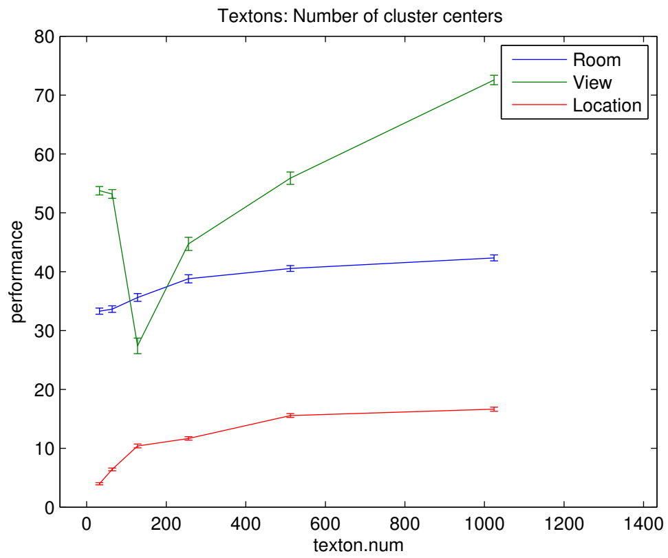
Figure 3. Texton performance by number of cluster centers.
