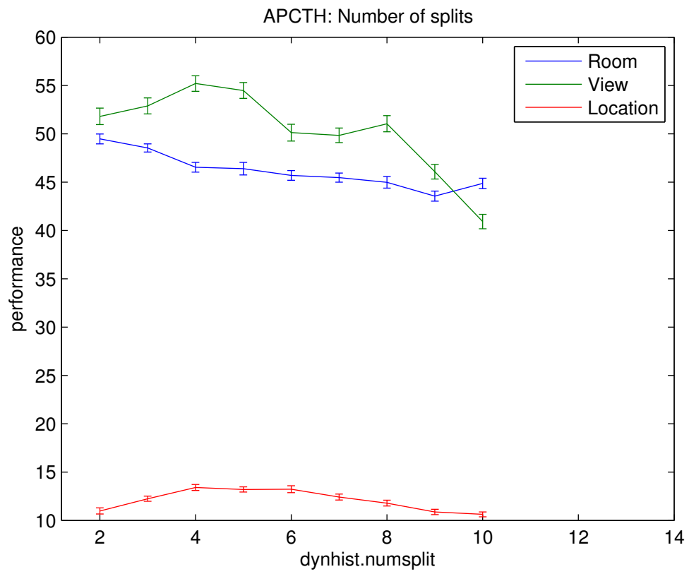
Figure 2. APCTH performance by number of partitions.
