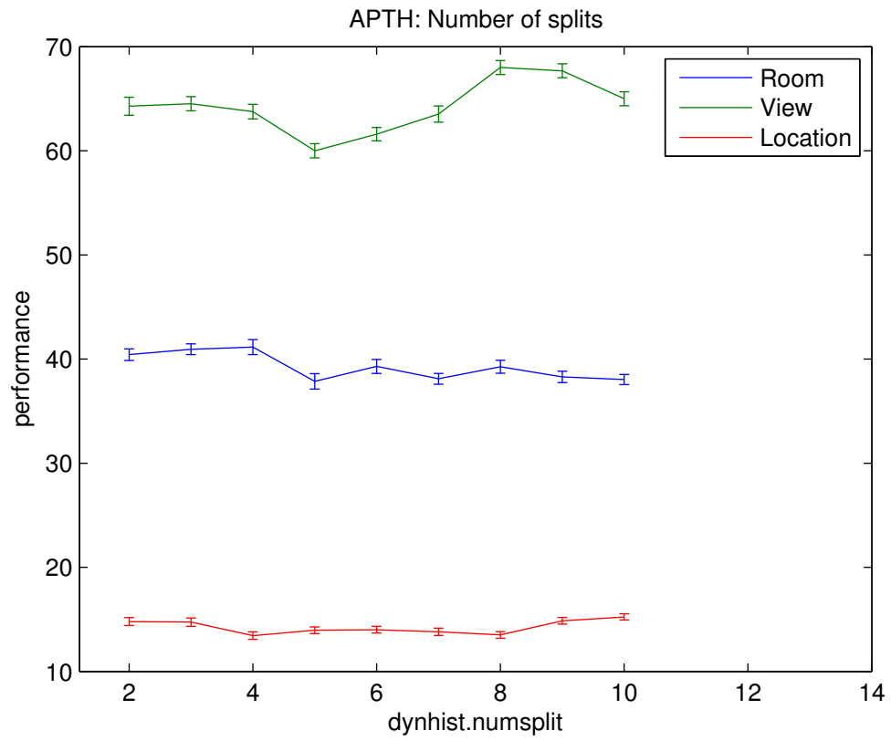
Figure 1. APTH performance by number of partitions.
