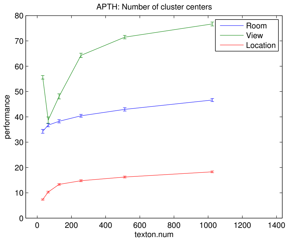
Figure 4. APTH performance by number of cluster centers.
